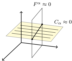
Figure 3: The reduced phase space is the intersection of the two surfaces.
