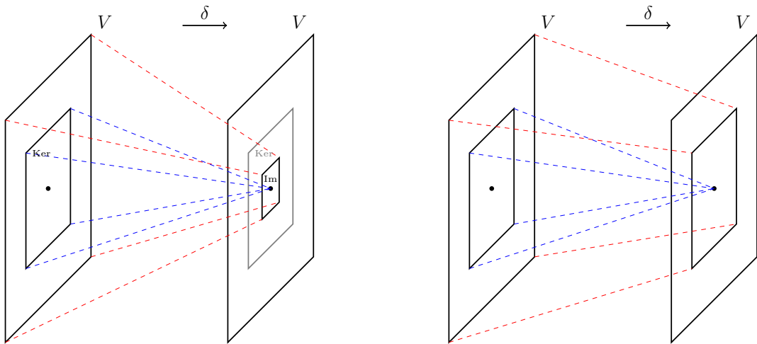
Figure 4: The cohomology measures the amount of non-exactness of closed elements. It is nontrivial when \text{Im}(\delta) \subset \text{Ker}(\delta) . The right hand side depicts the case of vanishing cohomology, \text{Im}(\delta) = \text{Ker}(\delta) and all closed elements are exact.
