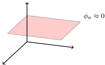
Figure 1: Phase space with the constraint surface identified by \phi_a \approx 0 .
