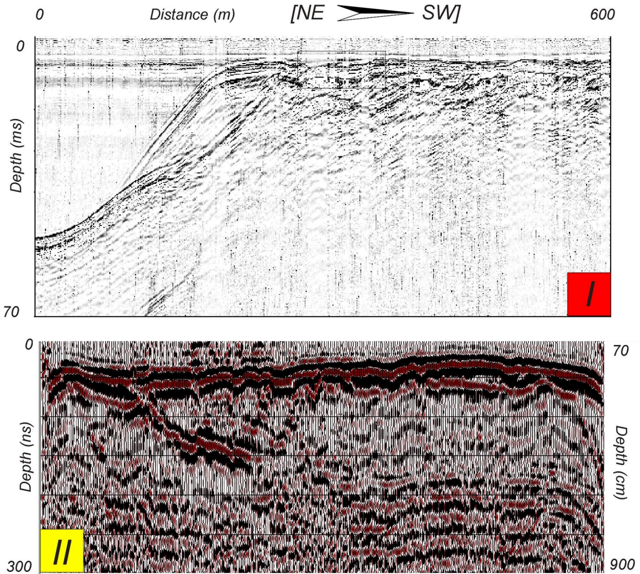
Figure 3: Comparison between I) 400 Hz bubble pulser profile and (II) 50 MHz GPR profile. The box in (I) indicates the zone of overlap.
